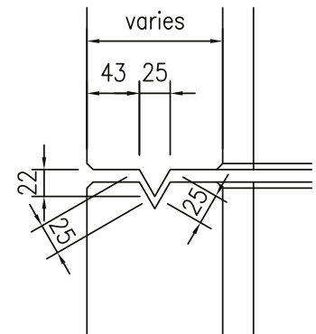
Joint Detail (1:5)
