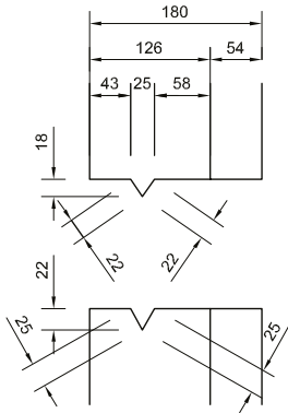
Joint Detail
