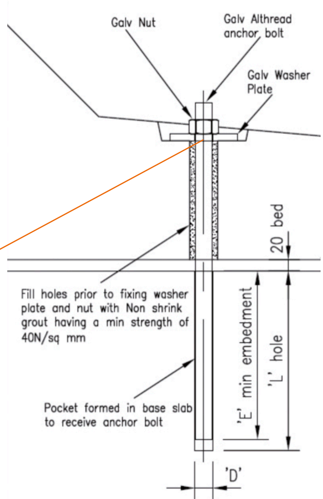
Anchor Bolt Detail
