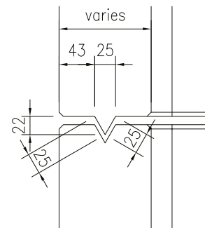
Joint Detail (1:5)
