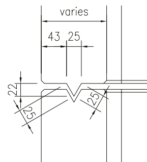
Joint Detail (1:5)
