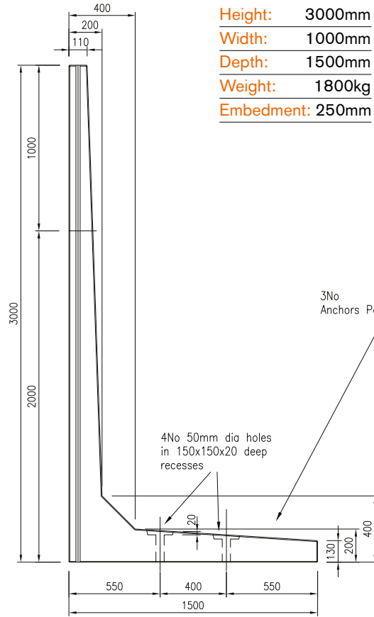
Side Elevation
