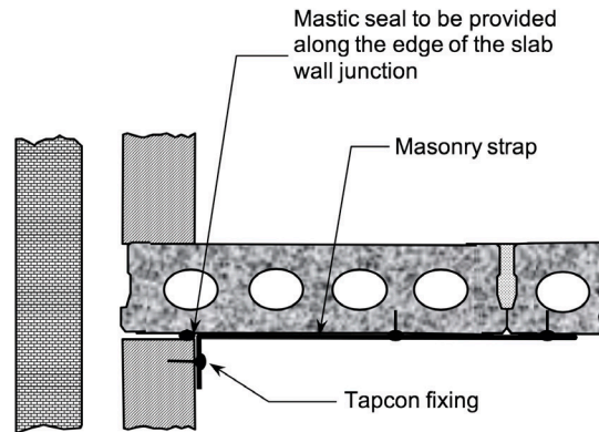
Figure 3 - Anchorage where a slab parallel to a wall is not bedded
